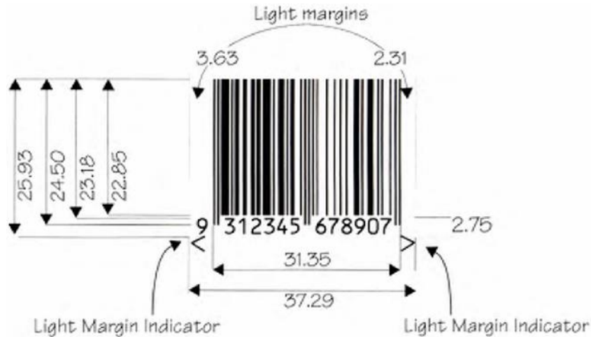
Figure 3: Dimensions in millimetres of an EAN-13 at 100% magnification (image not to scale)
