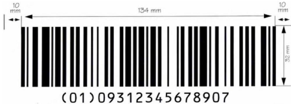
Figure 9: GS1-128 barcode dimensions at nominal (100%) magnification (not to scale)
